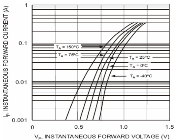
Fig. 1 Forward Characteristics
